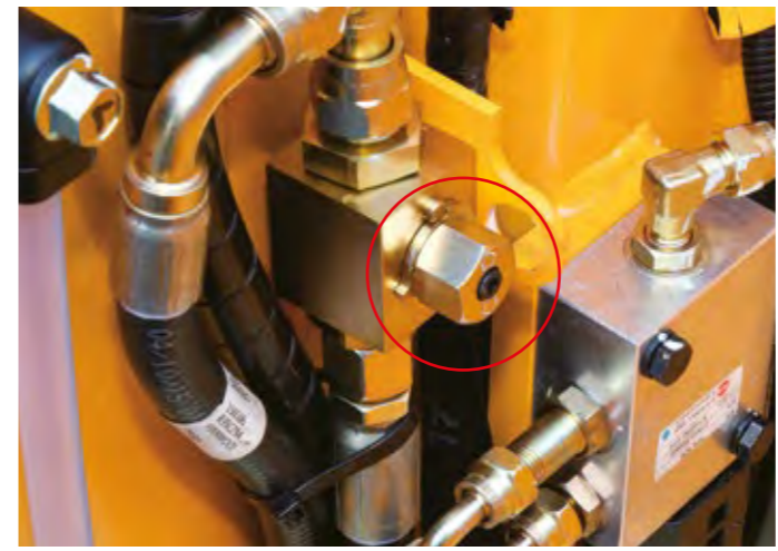
Selector valve for single or double acting pipe The double acting pipe located on front of the fuel tank assures easy access and control. Lever direction: vertical = single acting piping (breaker); horizontal = double acting piping (clamshell)
